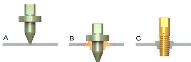
Flowdrillen
